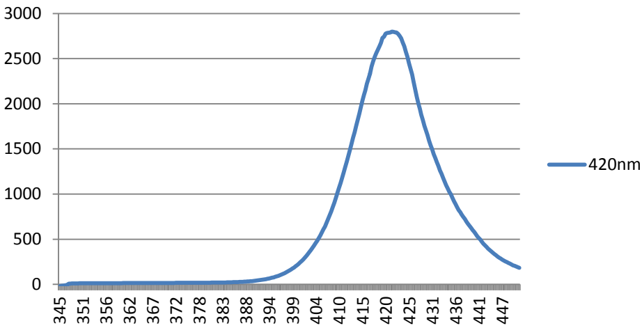
420nm LED Reefi Duo Extreme
