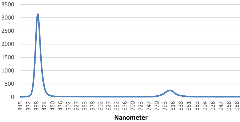
400nm LED in Reefi Exteme Luminaire
